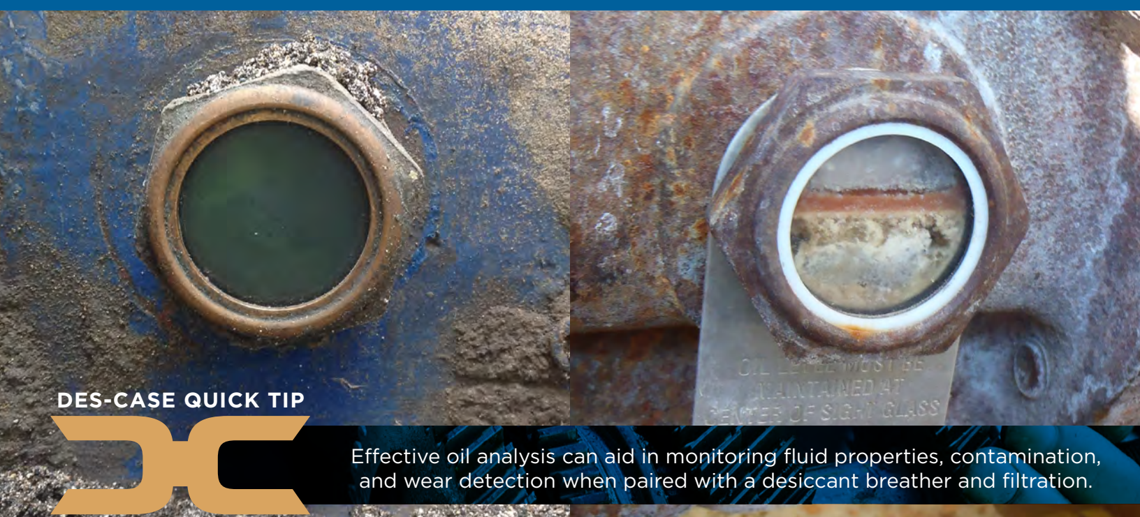
3-D BULLSEYE® VS. DIRTY OEM VIEWPORTS
